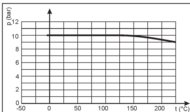
Fig. 5 - pressure-temperature diagram
