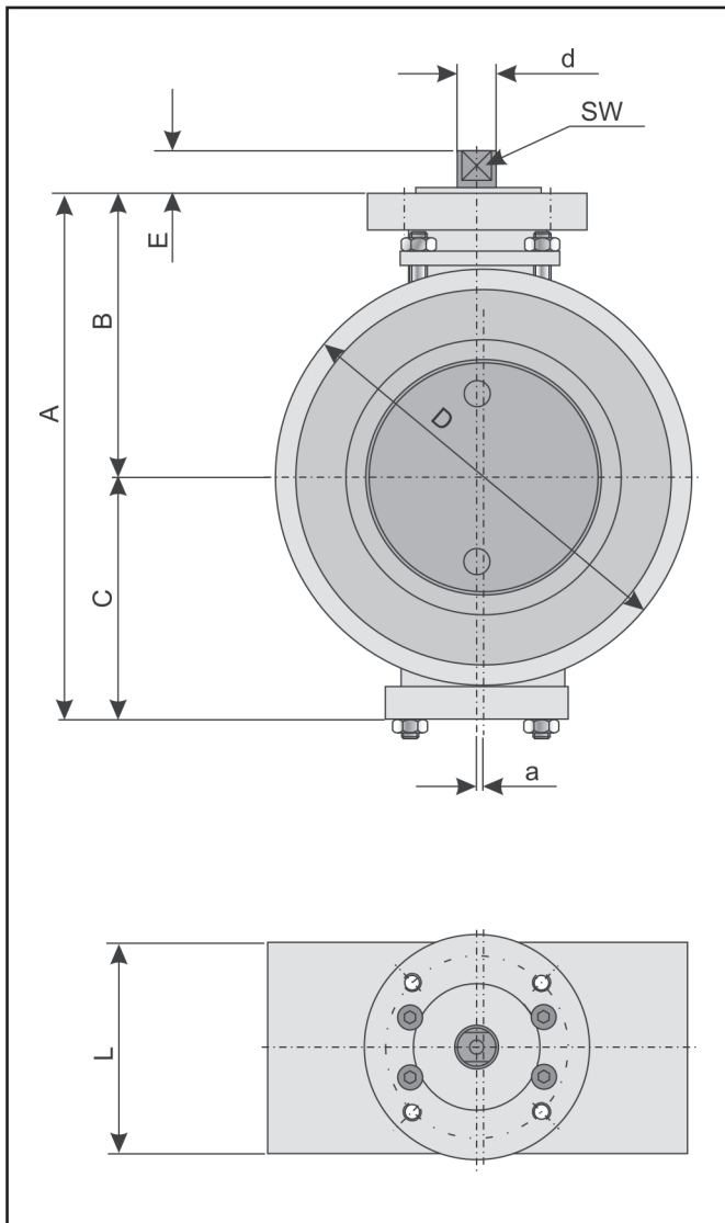
Fig. 7 – dimensional diagram
