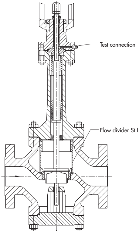
Fig. 4: Type 3254 Valve with flow divider St I and additional bellows seal with test connection
